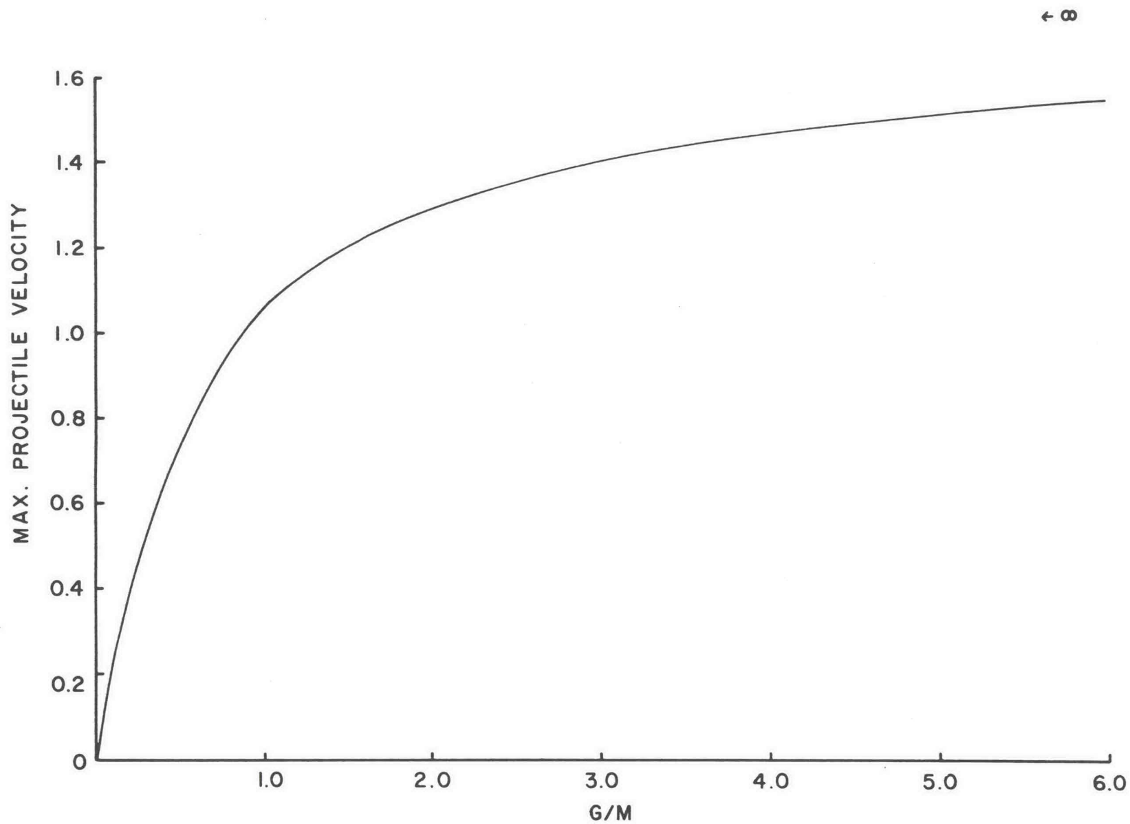
Fig. 2. Maximum projectile velocity as a function of G/M for 14 m barrel. Helium gas. (After Siegel 5 )
